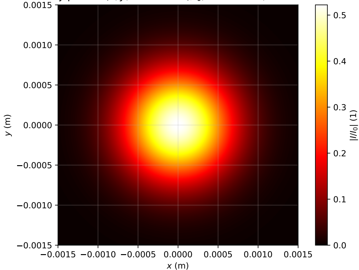
Intensity profile I(x, y, z = 2.070m)/I_0 , \text{Pin}=0.1\text{Pcr} , artificial time
